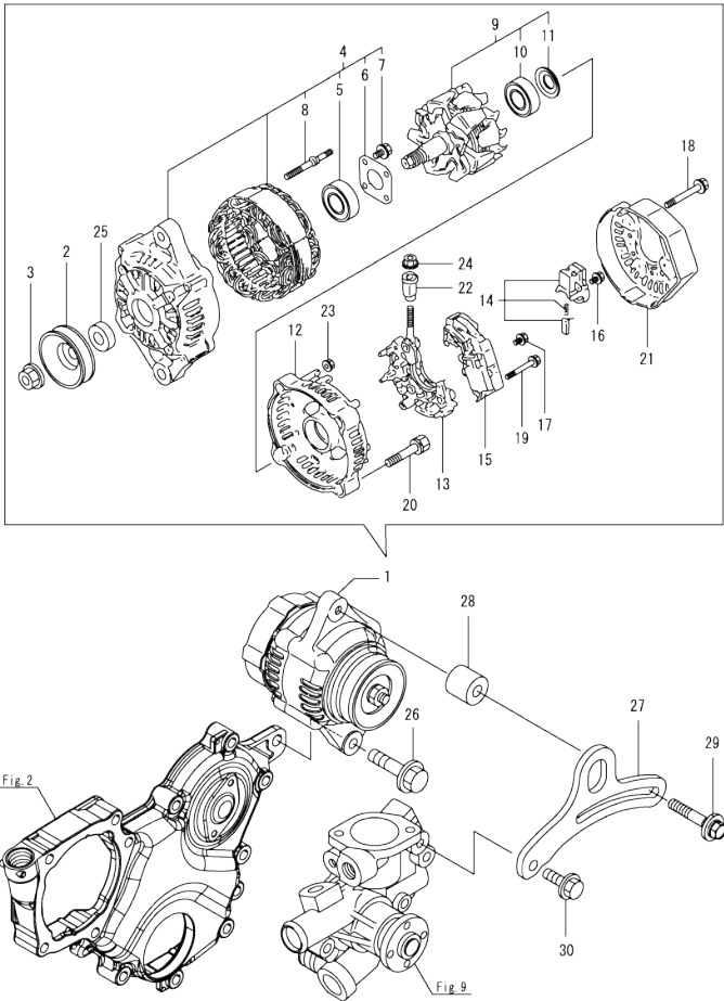
OCD50-M03660 ENGINE Fig.15. GENERATOR
